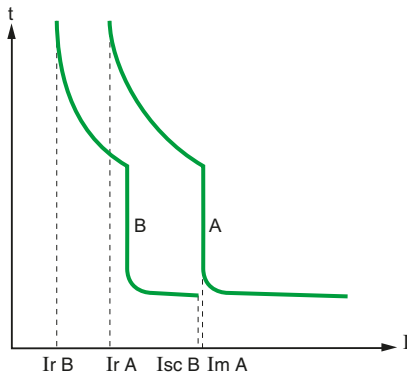
Total selectivity between CBs A and B.
