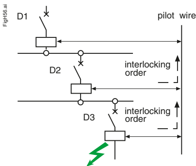
Logic selectivity
